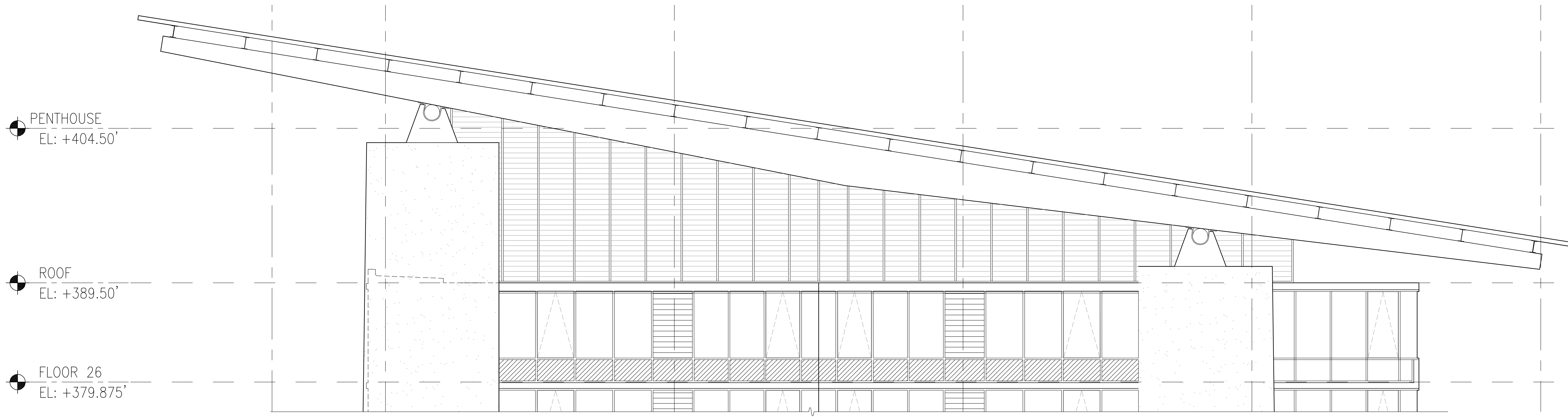
1 TOWER WEST PARTIAL ELEVATION SCALE: 1/4"=1'-0"
